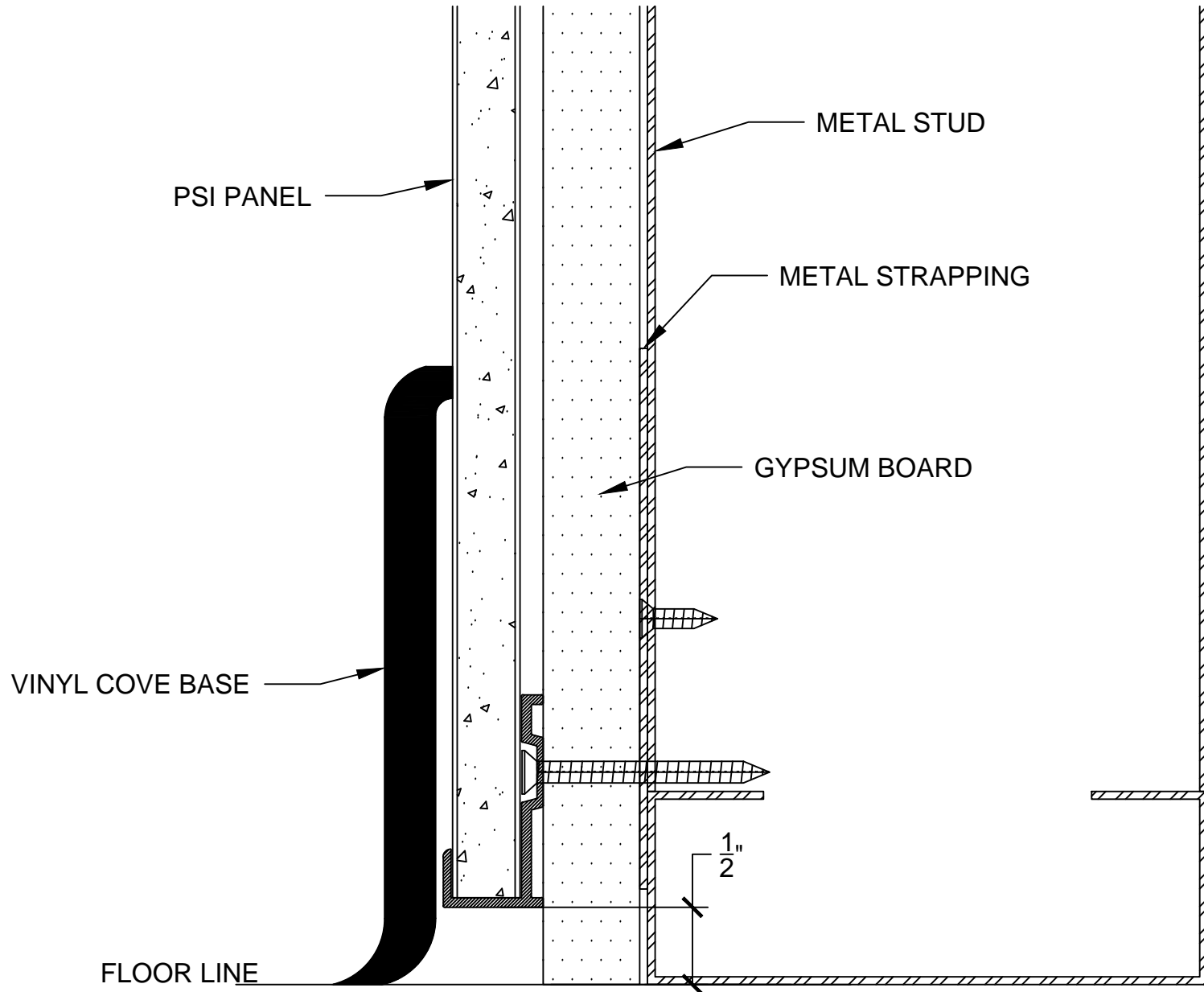
#610 BOTTOM EDGE TRIM - BEHIND BASE
