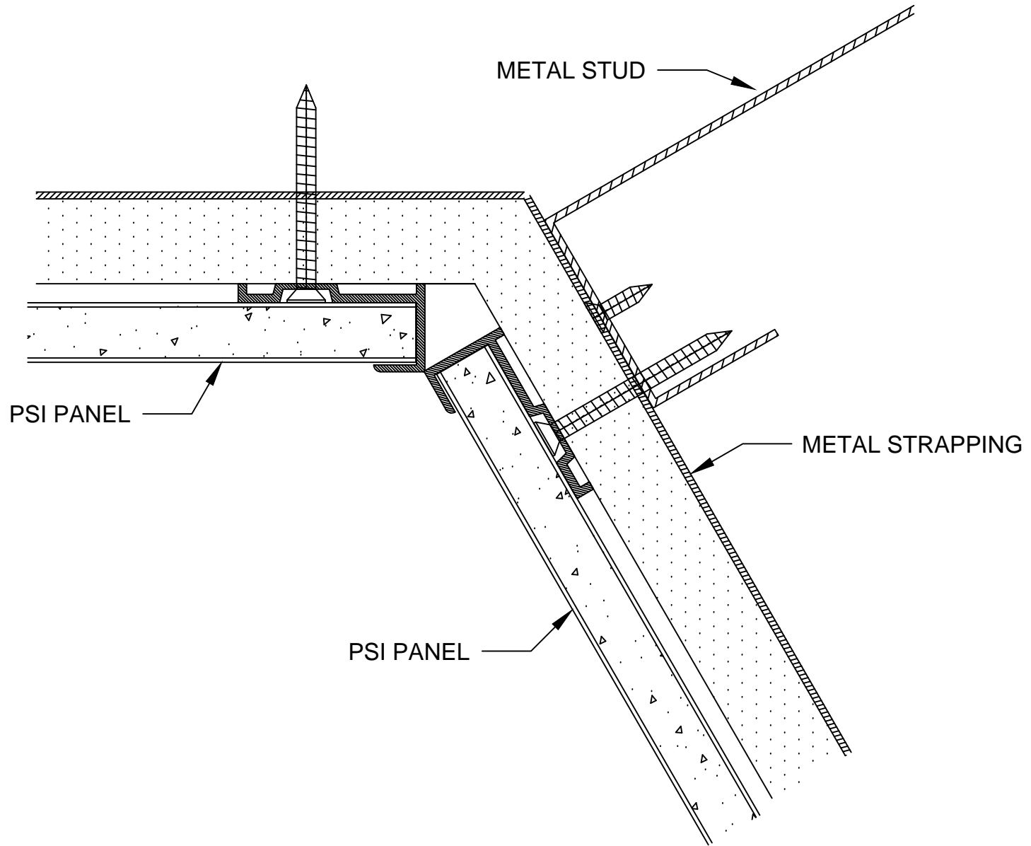
#610 ANGLED INSIDE CORNER TRIM
