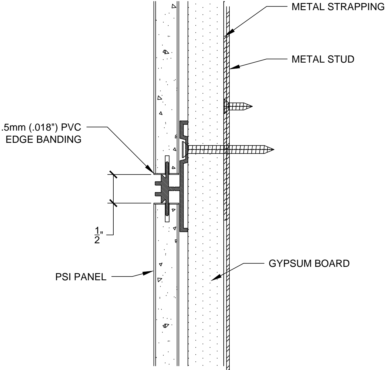
#632H HORIZONTAL REVEAL
