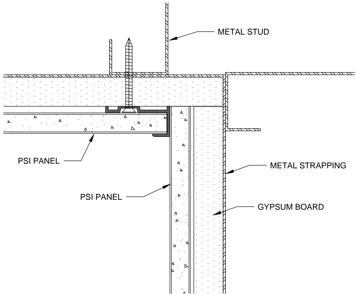
#610 INSIDE CORNER TRIM
